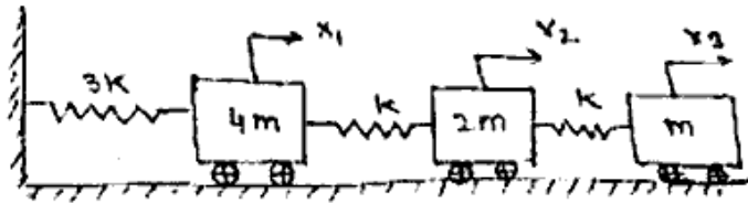
A Three degree of Freedom system 20
